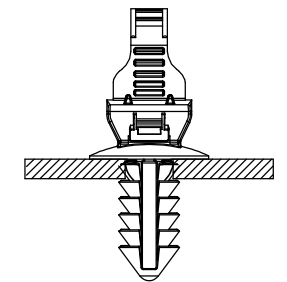
ASSEMBLED VIEW
